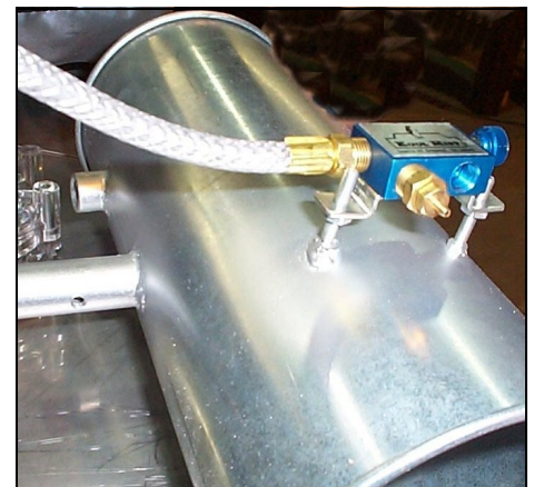
Model 2000 Silicone Mister System meters out the correct quantity of silicone
