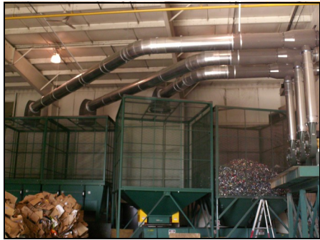
Paper, Plastic, Can, & Cardboard Recycling System with Energy Savings Venturi
